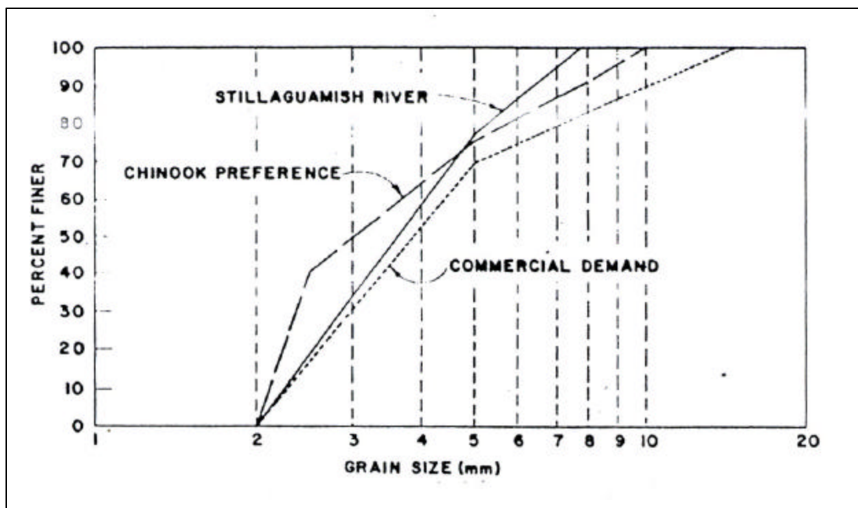
Figure 8. Diagram showing gravel sizes preferred by spawning salmonids and commercial gravel miners (Source: Bates 1987).
