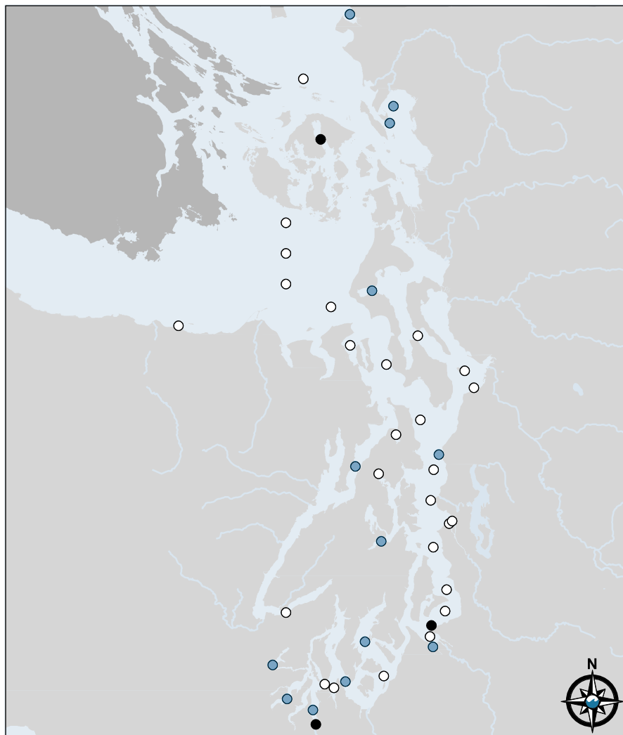
Figure 5-5. Maximum ammonium concentrations at marine monitoring stations in Puget Sound, 2001-2005.
