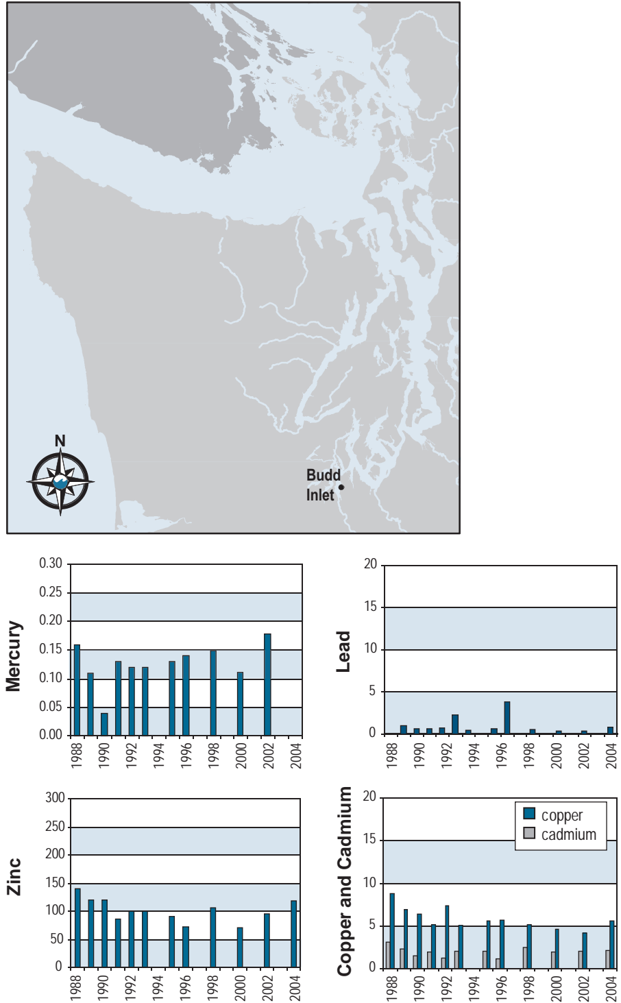
Figure 4-41e. Trends of metals in mussel tissue at Budd Inlet in Puget Sound.
