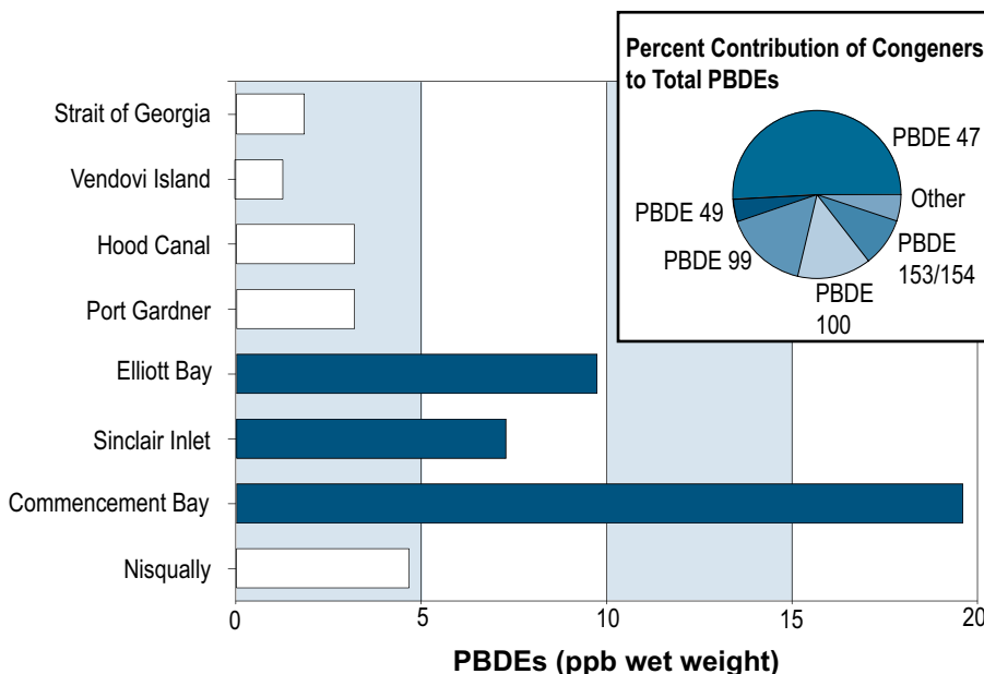
Figure 4-7. PBDE concentrations in English sole. Fish were sampled from three urban (shaded bar) and five non- or near-urban (open bar) Puget Sound locations in 2003.
