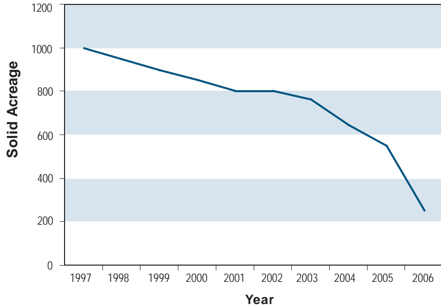
Figure 2-45. Decline in Spartina in Puget Sound. Successful efforts to remove the invasive seagrass will likely result in complete eradication by 2010.
