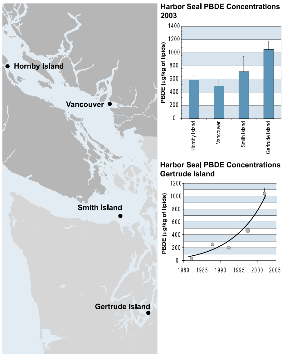
Figure 4-21. PBDEs in harbor seals from the Georgia Basin and Puget Sound. The map illustrates the locations of collection sites in 2003 near Hornby Island, Vancouver, B.C., Smith Island and Gertrude Island, and Puget Sound. Seals pups near Gertrude Island in Southern Puget Sound had nearly twice the PBDE levels of Vancouver seals (upper graph). Analysis of archived tissue (lower graph) shows the exponential increase in PBDEs since the early 1980s. (Source: WDFW and Fisheries and Oceans Canada)
