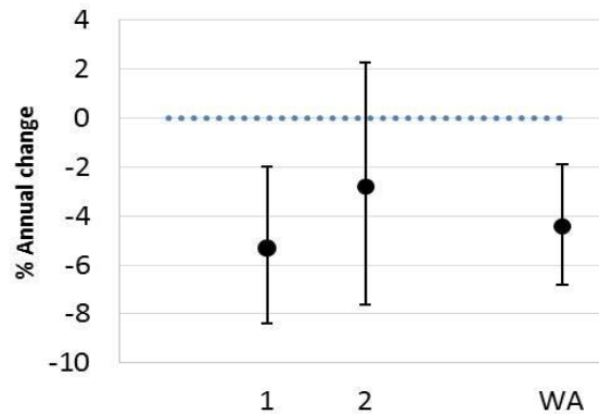
Figure 6. Marbled Murrelet population average rate of annual change from 2001-2015, with 95% confidence intervals for the Salish Sea (Zone 1), outer coast (Zone 2) and combined (WA). Dashed line (0) indicates stable population; intervals not overlapping 0 are significant (figure from Falxa et al. 2016b, used by permission).
