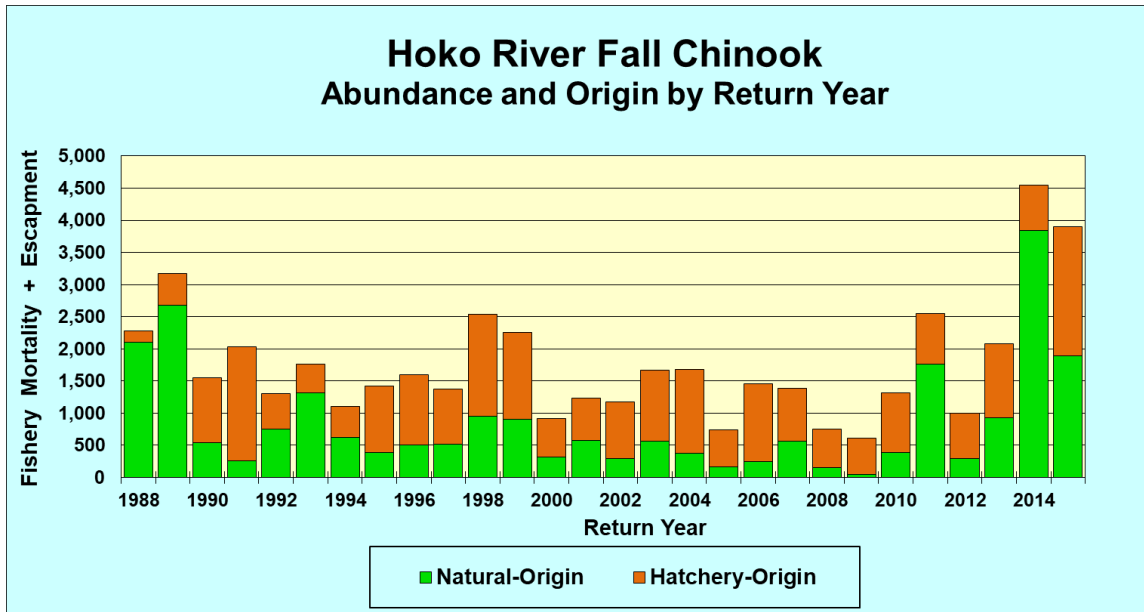
Figure 1. Hoko River Chinook, Abundance and Origin by Return Year. Over the long-term, slightly over half (58%) of the recruits have been of hatchery origin.
