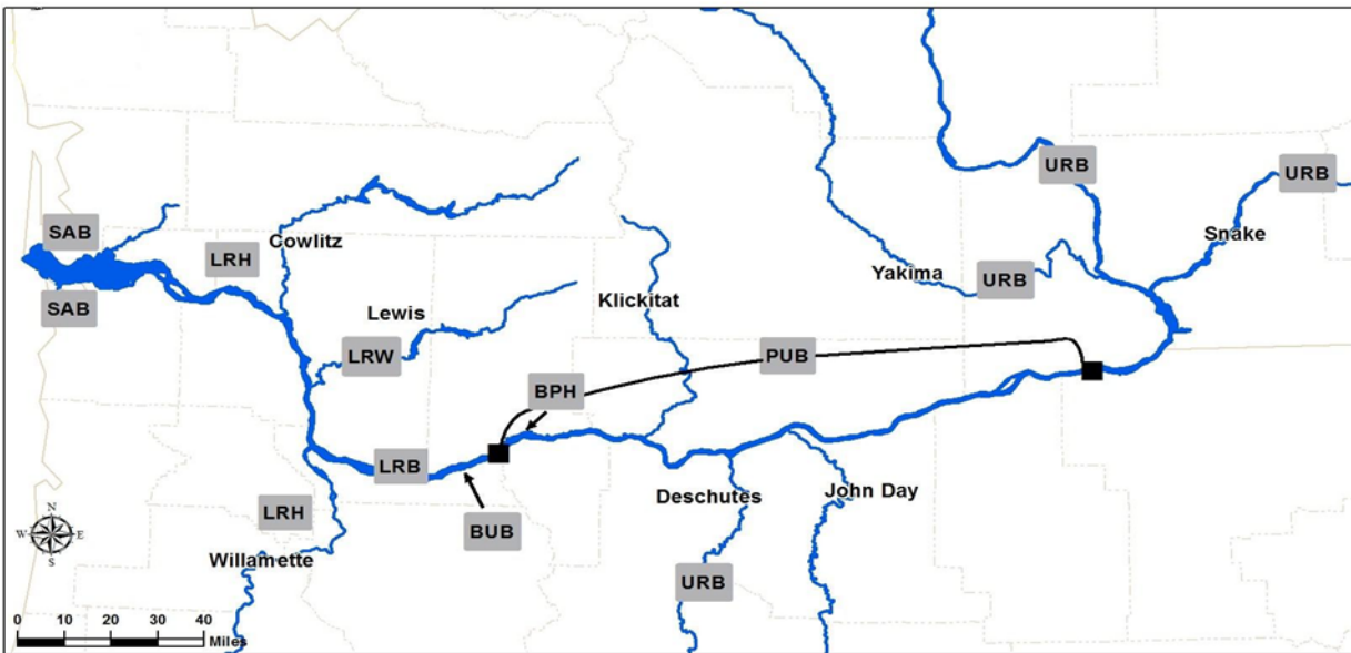
Figure 1. Major Columbia River fall Chinook stock components and general destinations.
