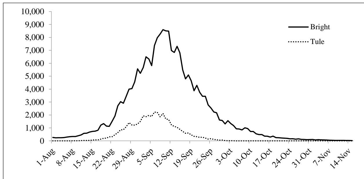
Figure 2. Ten-year average (2009-2018) daily passage of fall Chinook at Bonneville Dam.
