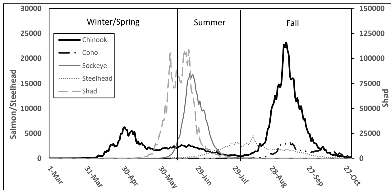
Figure 4. Ten-year average (2009-2018) of daily fish counts at Bonneville Dam.
