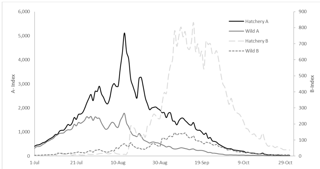
Figure 3. Ten-year average (2009-2018) daily passage of A- and B-Index summer steelhead at Bonneville Dam.
