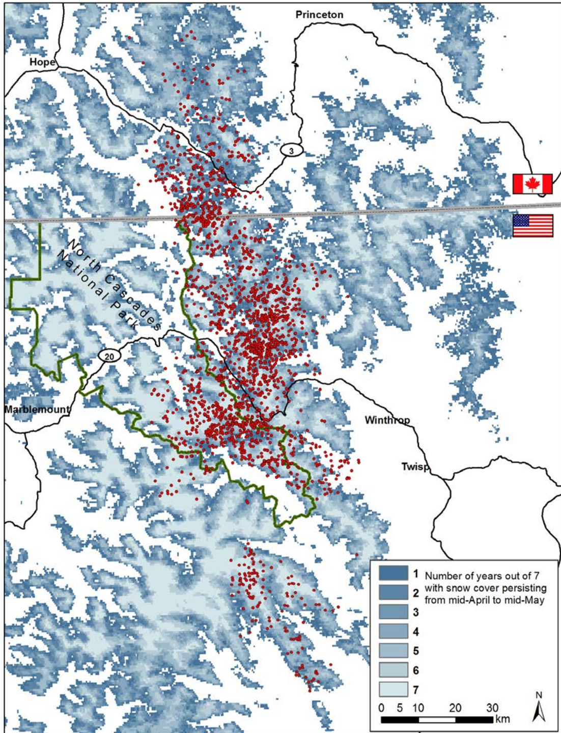
Figure 7. More than 2,000 high-quality satellite locations (red dots) obtained on 9 wolverines monitored from 2008/09 thru 2012/13 overlaid on a map of persistent spring snow cover developed by Copeland et al. (2010) and representing potential wolverine habitat in the Northern Cascades Ecosystem. Two wolverines that made long-distance movements are not included.
