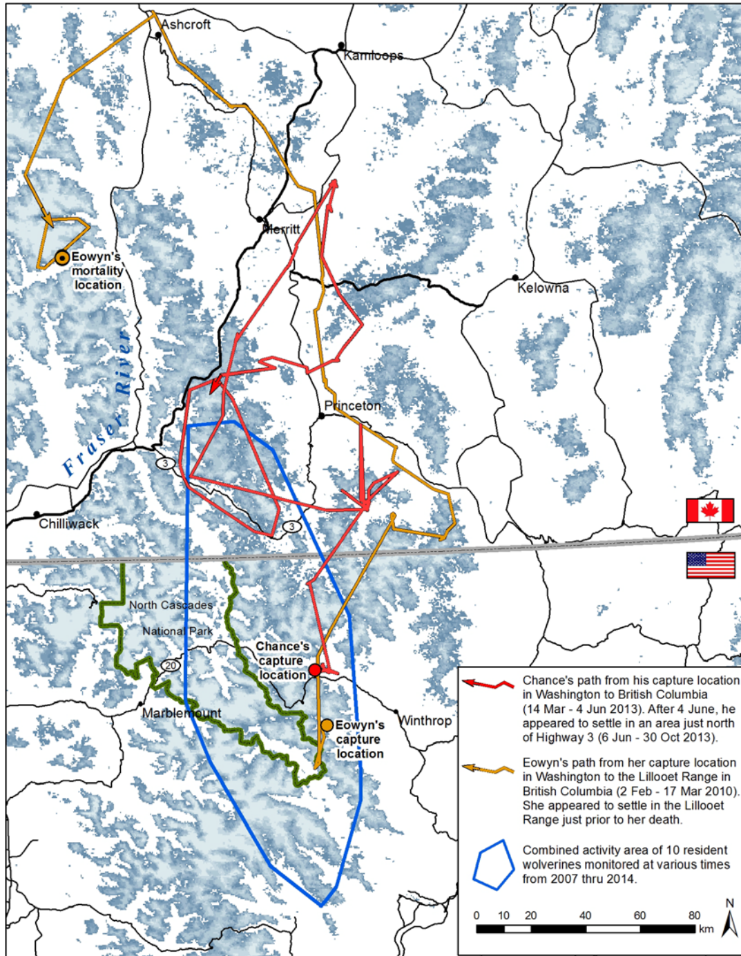
Figure 5. Long-distance movements made by a subadult male (Chance) during 2013 and a young nulliparous female wolverine (Eowyn) during 2010. Movement paths were determined using satellite location accuracy classes 3 (<250 m) and 2 (250-500 m). Polygons depicting areas of more localized movements, as well as the combined activity area for resident wolverines, were determined using satellite location accuracy classes 3, 2, and 1 (500-1500 m).
