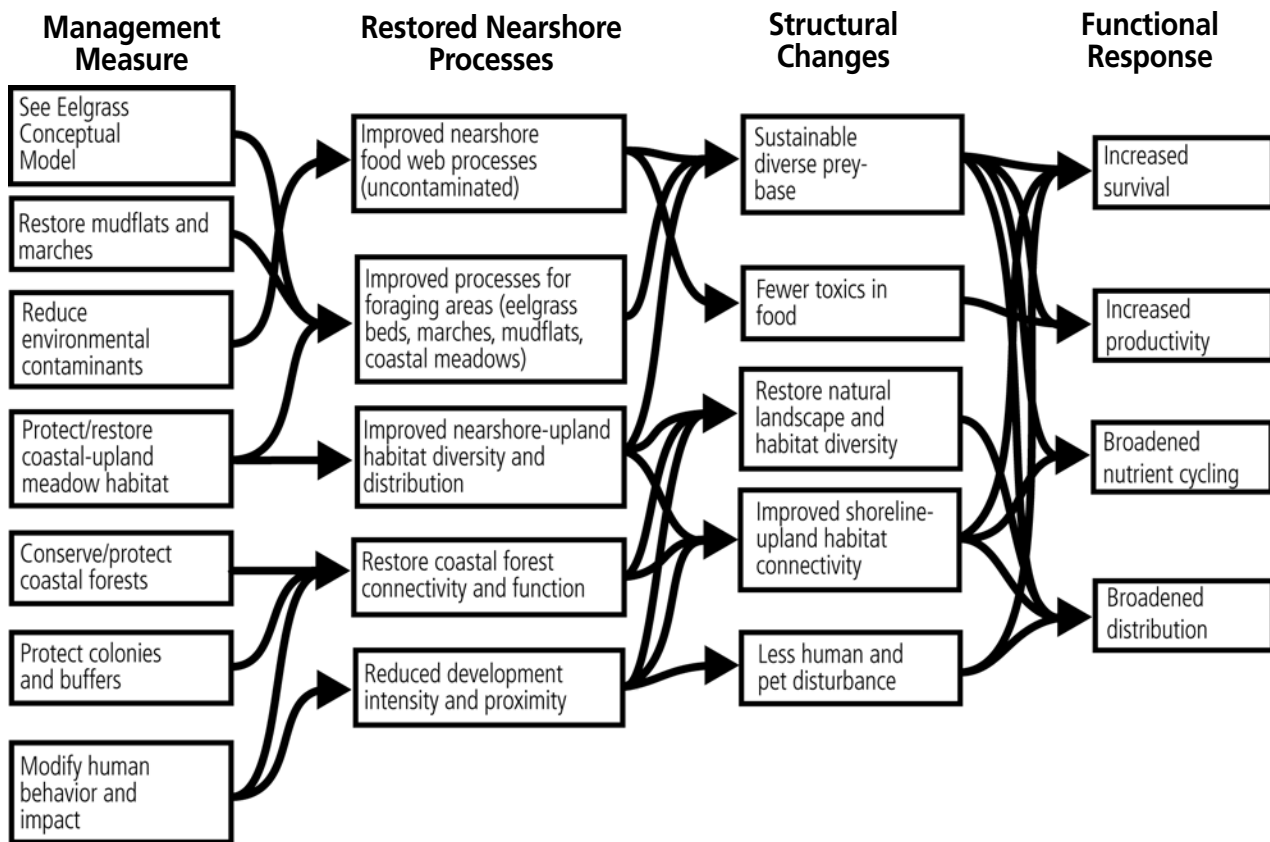
Figure 8. VEC model.
