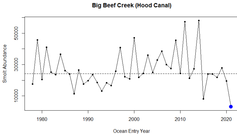
Figure 7. Time series of wild coho smolts from Big Beef Creek, ocean entry years 1978 to 2021. Blue point represents outmigration of the cohort included in this forecast. Horizontal line is the geometric mean of the time series.
