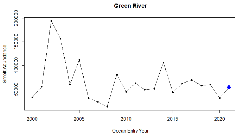
Figure 11. Time series of natural-origin coho smolts above the Green River smolt trap (river mile 34), ocean entry years 2000 to 2021. Blue point represents cohort contributing to this forecast. Horizontal line is the geometric mean for the time series.
