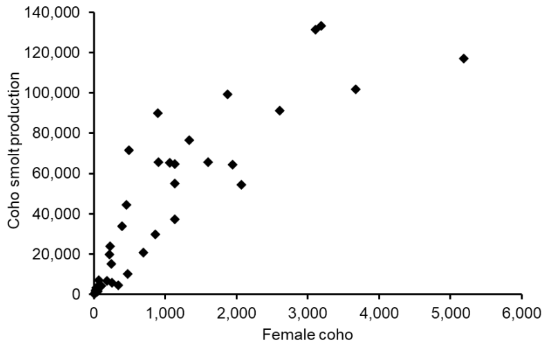
Figure 15. Coho smolt production as a function of female spawners in the Deschutes River, Washington, brood year 1978-2019.
