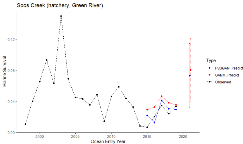
Figure 20. Marine survival of hatchery coho salmon released from Soos Creek hatchery in the Green River, ocean entry years 1998 to 2021. Black dashed line shows observed marine survival. Red dashed line (GAMM) and blue solid line (GAM) show marine survival estimated by one-step ahead forecasting. Solid blue point is the forecasted marine survival ( \pm 95\% C.I.) for the 2021 ocean entry year (2022 return year).
