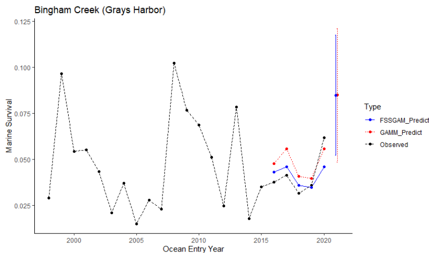
Figure 24. Marine survival of wild coho from Bingham Creek, Washington, ocean entry year 1998 to 2021. Black dashed line shows observed marine survival. Red dashed line (GAMM) and blue solid line (GAM) show marine survival estimated by one-step ahead forecasting. Solid blue point is the forecasted marine survival (±95% C.I.) for the 2021 ocean entry year (2022 return year).
