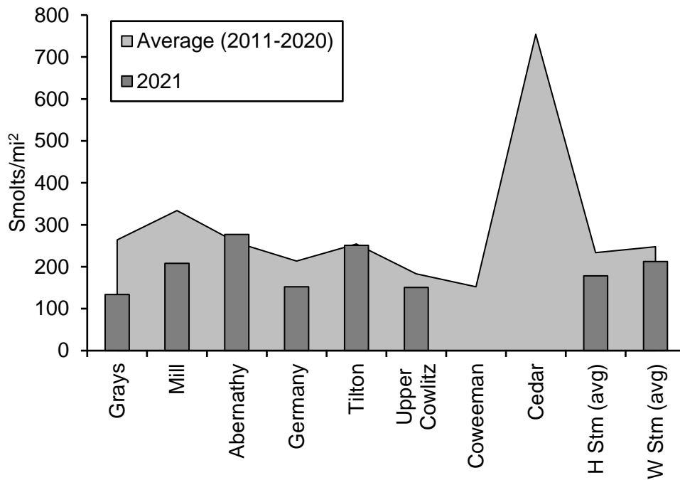
Figure 17. Coho smolt densities (smolts per mile 2 of watershed area) in eight Lower Columbia tributaries in Washington State. Graphs shows the 2021 density (bars) relative to the average smolt abundance from these watersheds (2011-2020).
