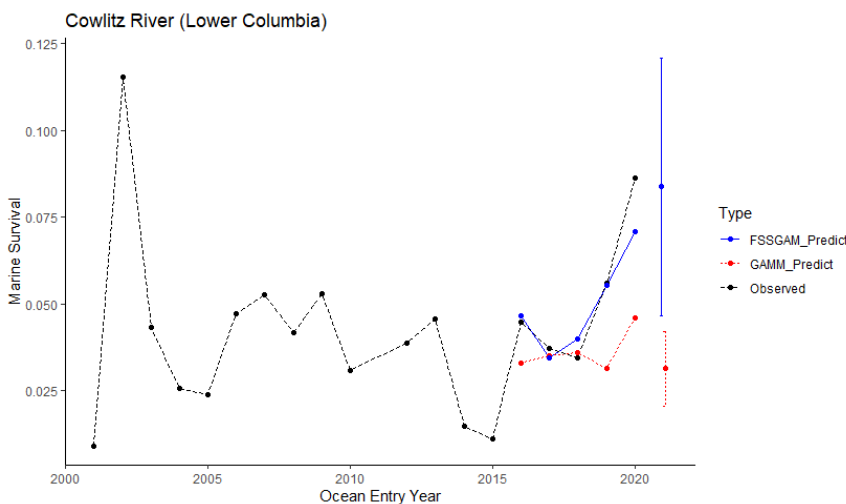
Figure 25. Marine survival of natural coho from the Lower Columbia River management unit, ocean entry year 2001 to 2021 (no marine survival data available for 2011). Black dashed line shows observed marine survival. Red dashed line (GAMM) and blue solid line (GAM) show marine survival estimated by one-step ahead forecasting. Solid blue point is the forecasted marine survival ( \pm 95\% C.I.) for the 2021 ocean entry year (2022 return year).
