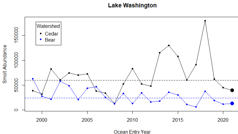
Figure 10. Time series of natural-origin coho smolts from Cedar River (black) and Bear Creek (blue), ocean entry years 1999 to 2021. Larger symbol represents outmigration of cohort contributing to this forecast. Horizontal lines are the geometric mean for the time series in each watershed.
