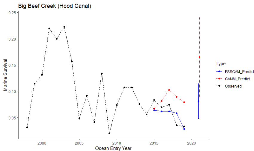
Figure 22. Marine survival of Big Beef Creek wild coho, ocean entry year 1998 to 2021. Black dashed line shows observed marine survival. Red dashed lone (GAMM) and blue solid line (GAM) show marine survival estimated by one-step ahead forecasting. Solid blue point is the forecasted marine survival ( \pm 95\% C.I.) for the 2021 ocean entry year (2022 return year).
