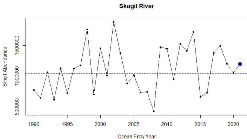
Figure 4. Time series of wild coho smolt outmigration from the Skagit River, ocean entry years 1990 to 2021. Blue point represents outmigration of the cohort included in this forecast. Horizontal line is the geometric mean of the time series.
