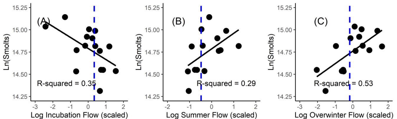
Figure 16. Chehalis River wild coho smolt production as a function of incubation flows (a), summer rearing flows (b), and overwinter rearing flows (c) for ocean entry year 2001-2021 as measured at USGS gage #12027500 in Grand Mound. Incubation flows are the cumulative daily mean flow between December 1 and March 1. Summer rearing flows are maximum daily flows in the month of August. Overwinter rearing flows are minimum daily flows between November 1 and February 28. Three data points were removed (OEY 2004, 2006, and 2015) because of high leverage on the regressions. Vertical blue dashed line indicates the conditions associated with the 2021 ocean entry year.
