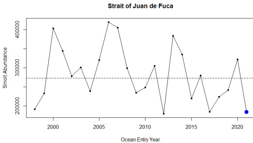
Figure 8. Time series of wild coho smolts from Strait of Juan de Fuca tributaries, ocean entry years 1998 to 2021. Blue point represents the cohort contributing to this forecast. The horizontal line is the geometric mean of the time series. Data provided by Hap Leon (Makah Tribe).
