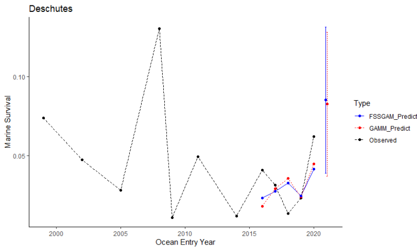
Figure 21. Marine survival of Deschutes River natural coho salmon, ocean entry years 1998 to 2021 (excluding years for which no marine survival data were available). Black dashed line shows observed marine survival. Red dashed line (GAMM) and blue solid line (GAM) show marine survival estimated by one-step ahead forecasting. Solid blue point is the forecasted marine survival ( \pm 95\% C.I.) for the 2021 ocean entry year (2022 return year).
