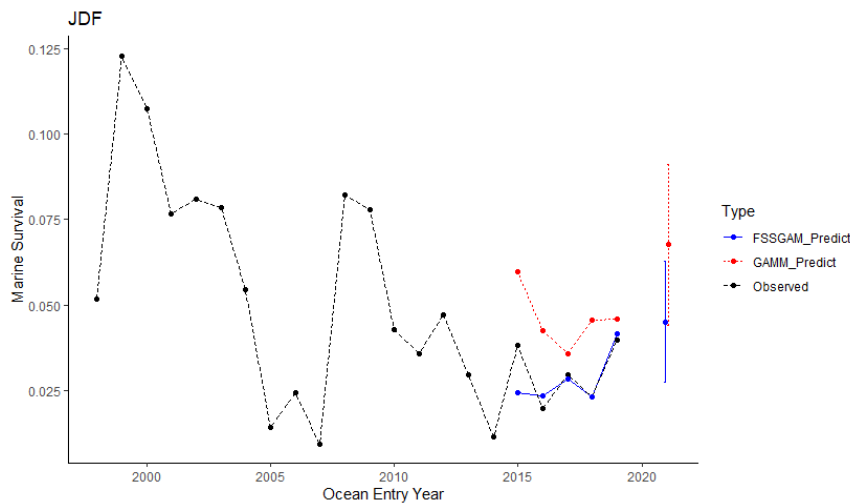
Figure 23. Marine survival of wild coho in the Strait of Juan de Fuca management unit, ocean entry year 1998 to 2021. Black dashed line shows observed marine survival. Red dashed line (GAMM) and blue solid line (GAM) show marine survival estimated by one-step ahead forecasting. Solid blue point is the forecasted marine survival (±95% C.I.) for the 2021 ocean entry year (2022 return year).
