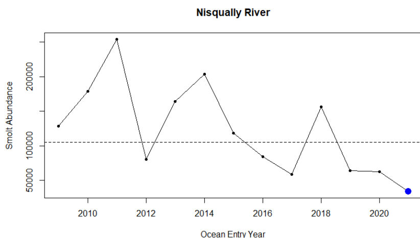
Figure 13. Time series of natural-origin coho smolts from the Nisqually River above the smolt trap (rm 12), ocean entry years 2009 to 2021. Blue point represents outmigration of the cohort included in this forecast. Horizontal line is the geometric mean for the time series.
